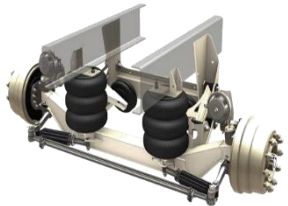
Lift Axle
